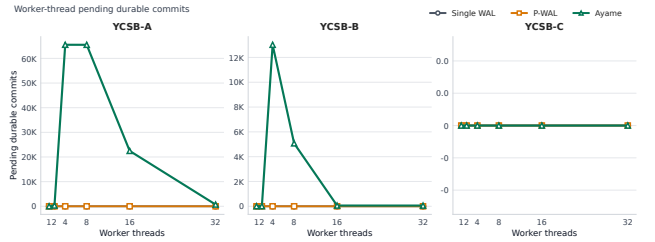
Fig. 4 Pending durable commits by transaction worker threads.
