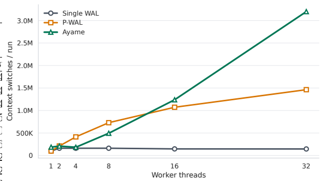
Fig. 8 Context-switch counts in the YCSB-B perf-stat worker-scaling runs.
