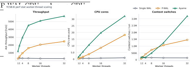
Fig. 9 Perf-stat summary for YCSB-B worker scaling.
