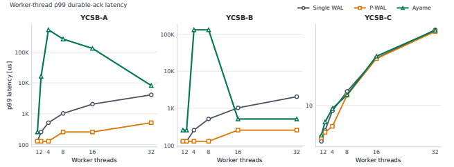
Fig. 3 P99 durable-acknowledgment latency by transaction worker threads.
