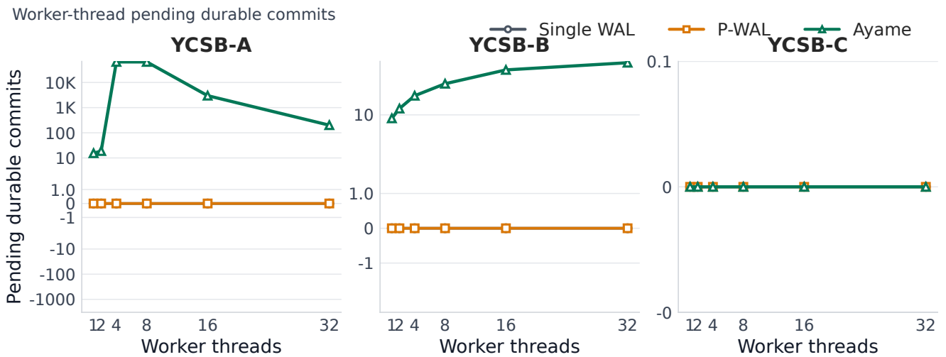
Fig. 4 Pending durable commits by transaction worker threads.
