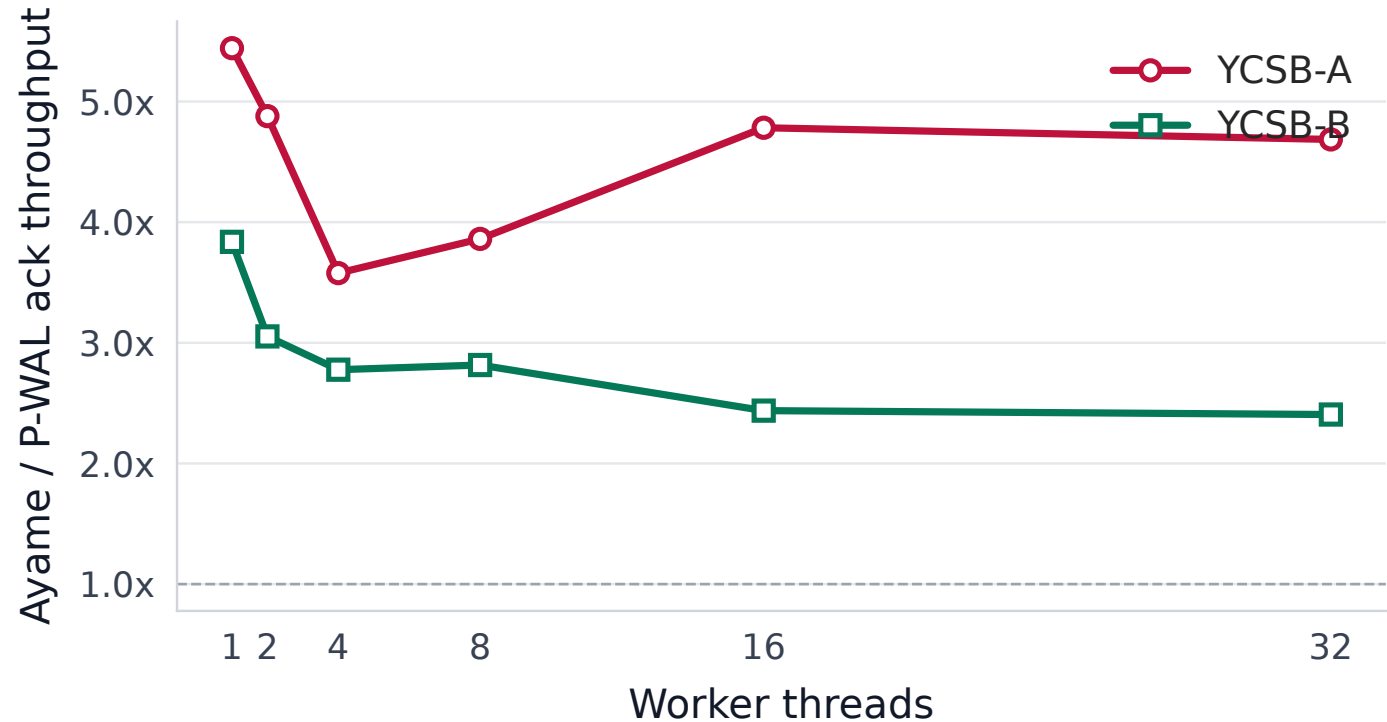
Worker-thread scaling; all modes use the same CCBench binary
