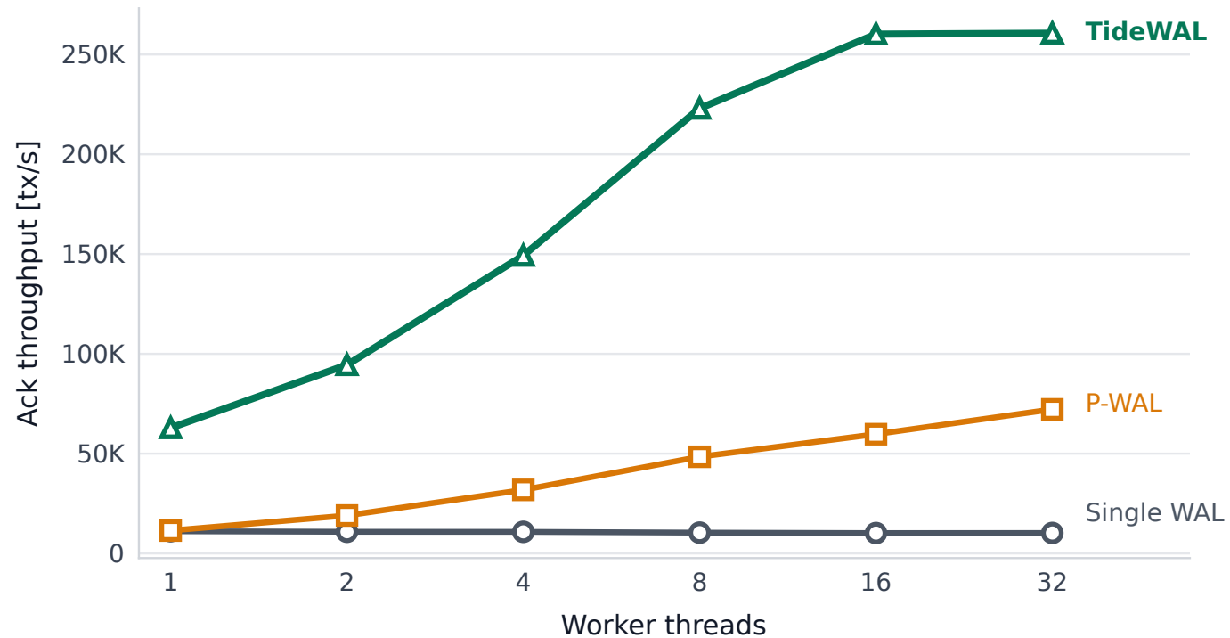
YCSB-A, 50% reads, 10 operations per transaction
