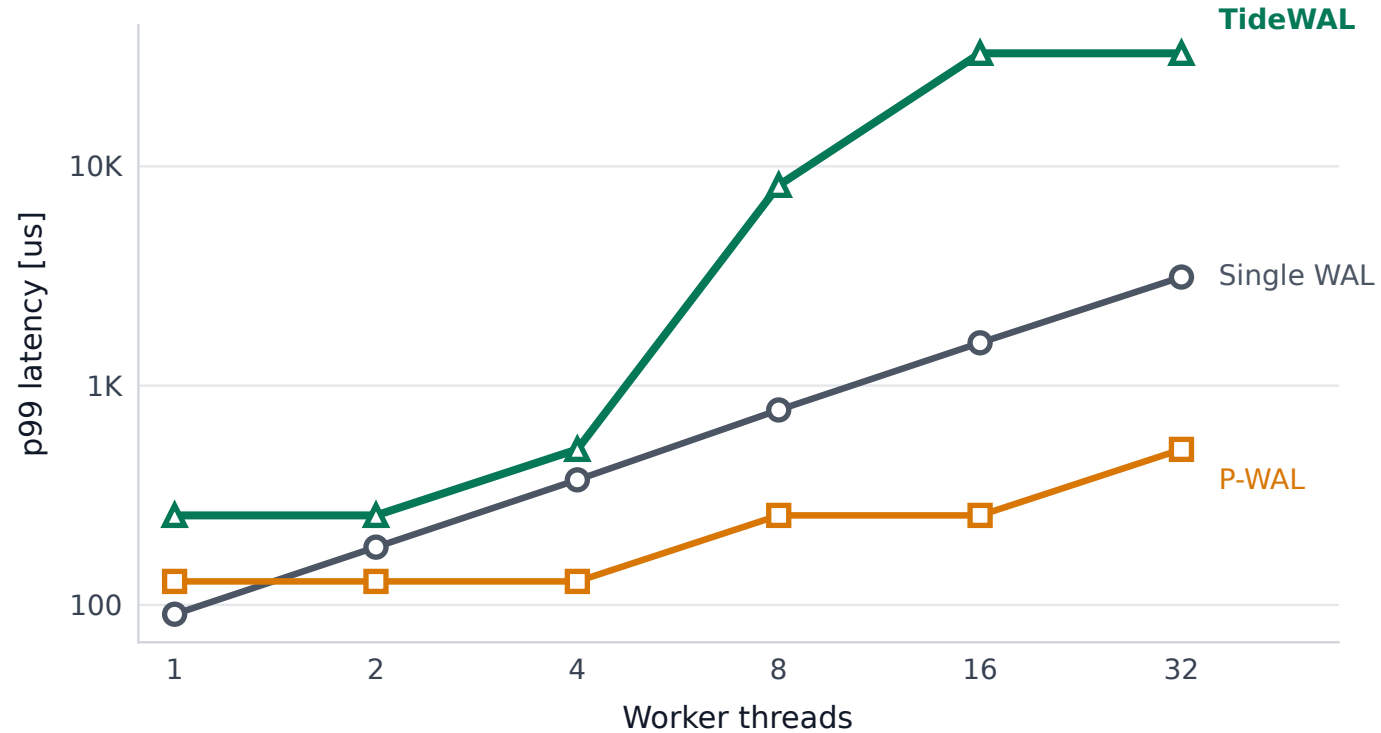
YCSB-A, p99 durable-ack latency
