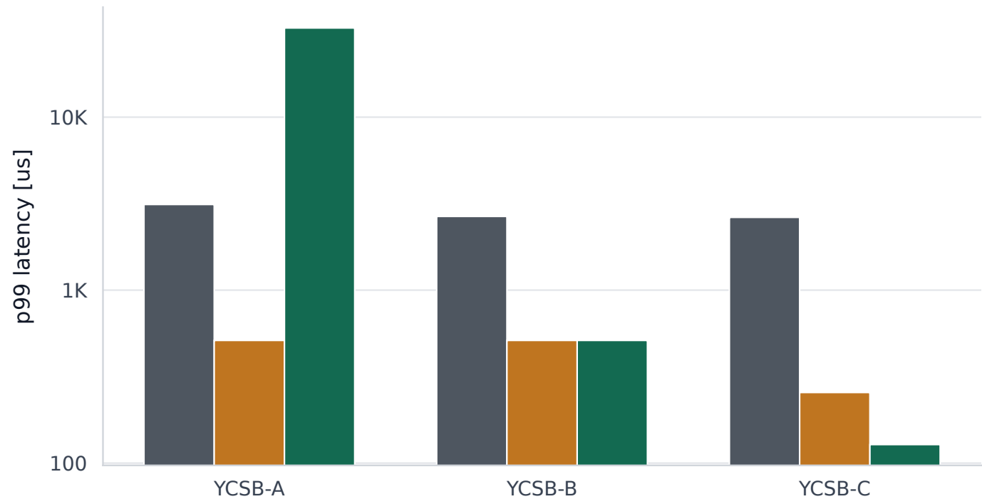
32 worker latencies across workload mixes
