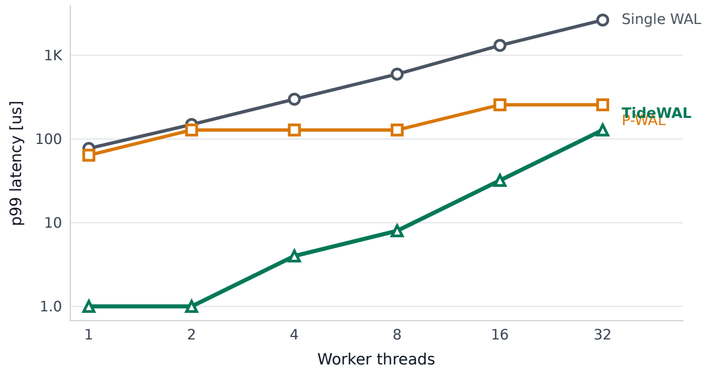
YCSB-C, p99 durable-ack latency
