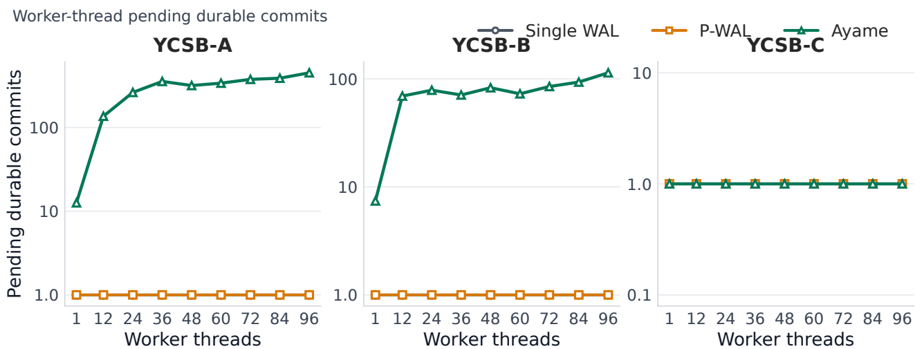
Fig. 4 Pending durable commits by transaction worker threads (log scale). Single WAL and P-WAL are synchronous and keep no pending durable commits; they are drawn at the axis floor.
