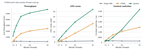
Fig. 9 Perf-stat summary for YCSB-B worker scaling.
