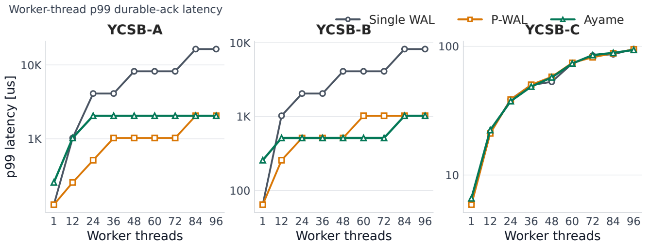
Fig. 5 P99 durable-acknowledgment latency by transaction worker threads.
