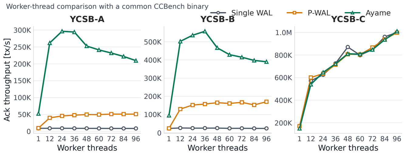
Fig. 3 Durable-acknowledgment throughput by transaction worker threads. Ayame improves update and mixed read-write workloads by combining parallel WAL logging, dependency-closed durable acknowledgment, and timestamp-integrated logical ordering.
