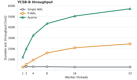
Fig. 6 YCSB-B durable-acknowledgment throughput in the perf-stat worker-scaling runs.
