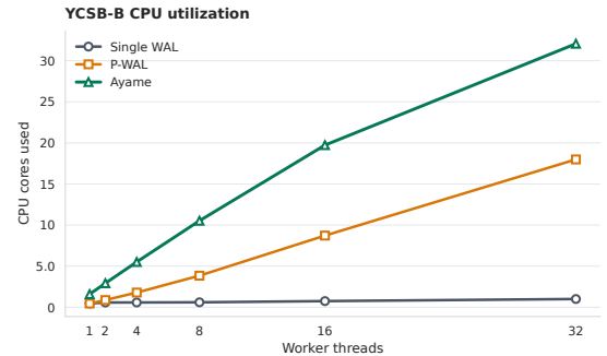
Fig. 7 CPU-core utilization in the YCSB-B perf-stat worker-scaling runs.
