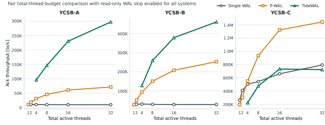
図 2 Durable-acknowledgment throughput under a fair total active-thread budget. TideWAL improves update and mixed read-write workloads by combining parallel WAL logging, dependency-closed durable acknowledgment, and timestamp-integrated logical ordering.
