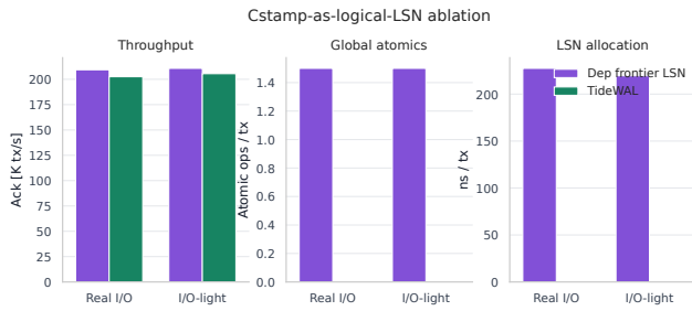
図 7 Cstamp-as-logical-LSN ablation.
