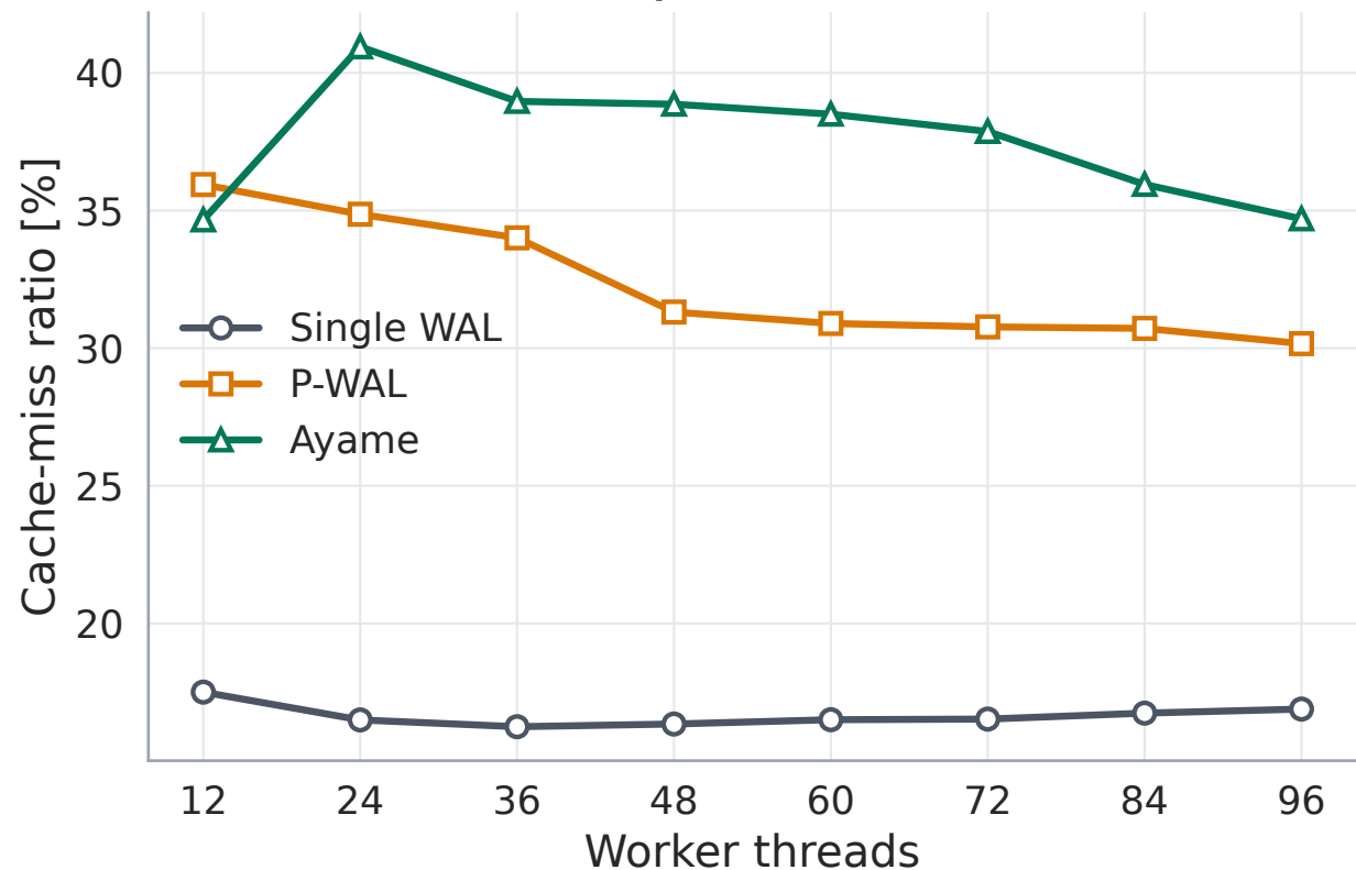
YCSB-A cache-miss ratio (cache-misses / cache-references)
