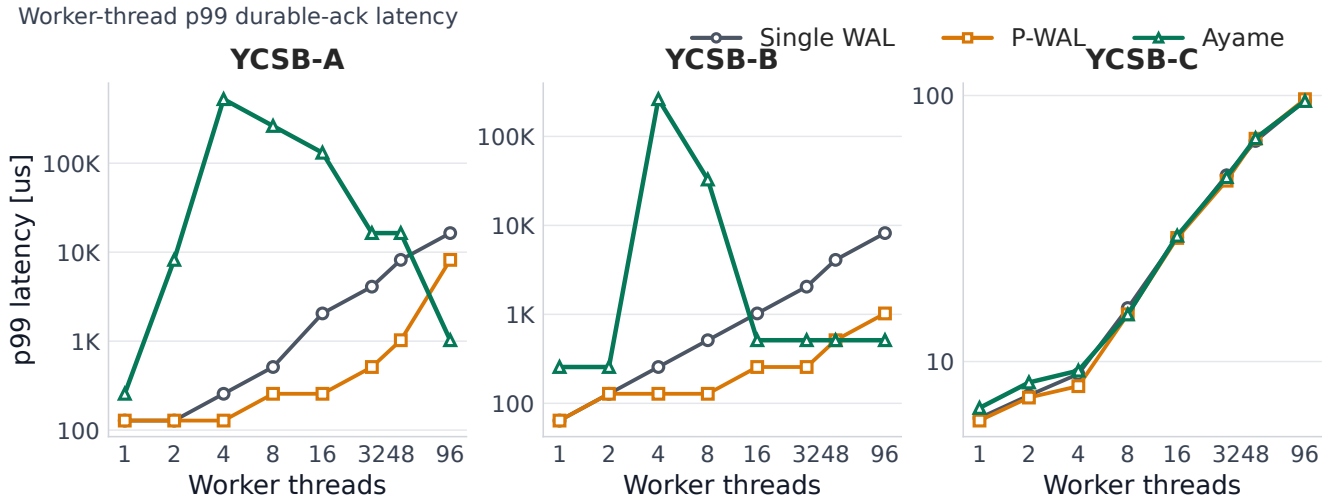
Fig. 3 P99 durable-acknowledgment latency by transaction worker threads.
