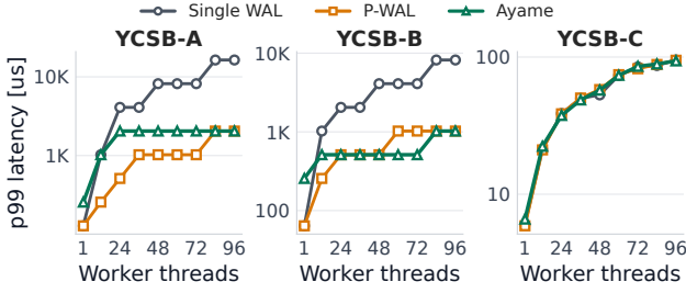
Fig. 4 P99 durable-acknowledgment latency by transaction worker threads.
