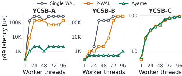
Fig. 3 P99 durable-acknowledgment latency by transaction worker threads.
