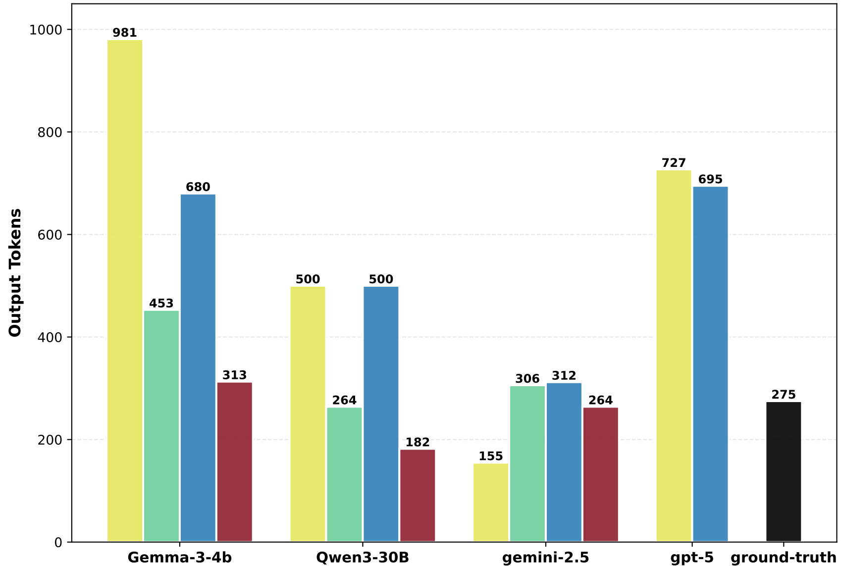
Output Tokens by Model and Approach (TB)
