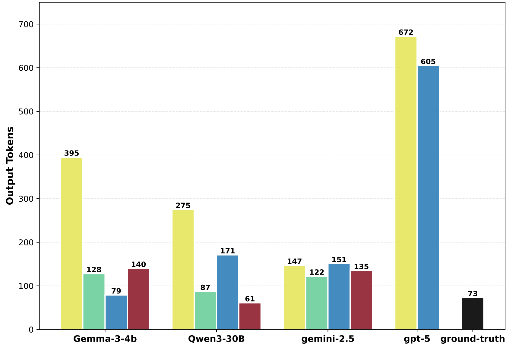
Output Tokens by Model and Approach (CD)
