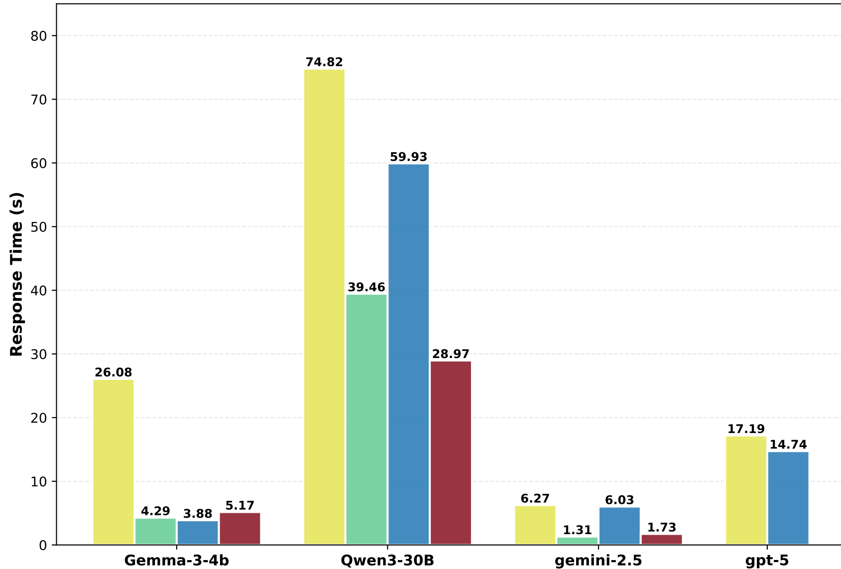
Response Time by Model and Approach (CD)
