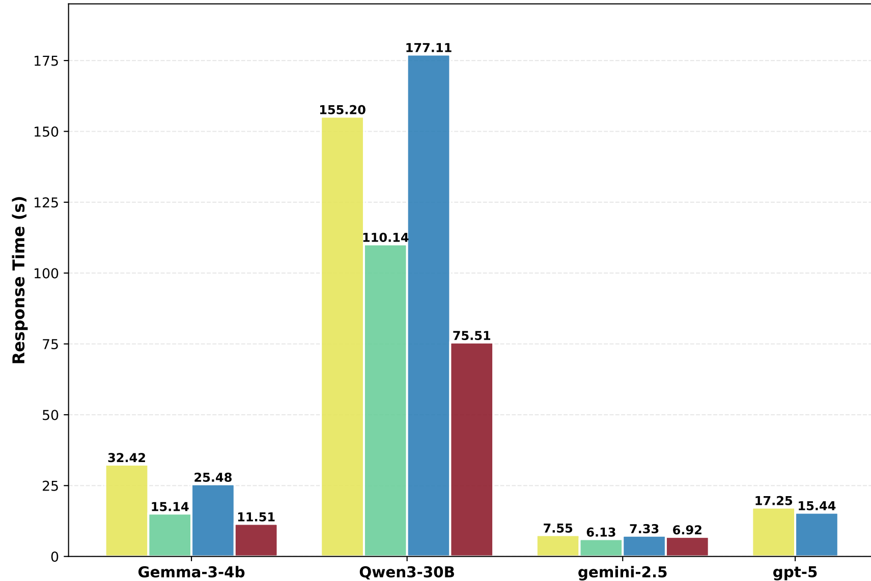
Response Time by Model and Approach (TB)
