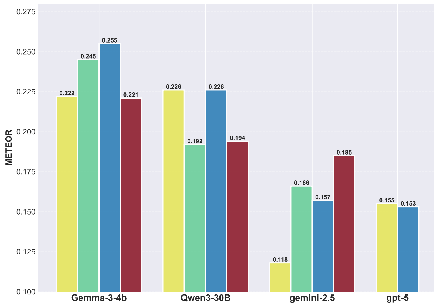
METEOR
