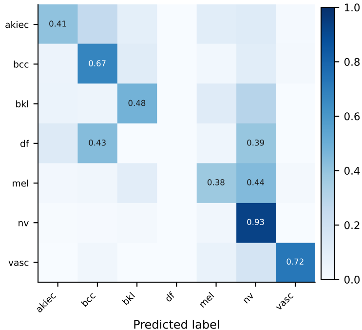
a) dermaMNIST (ACC=0.774)
