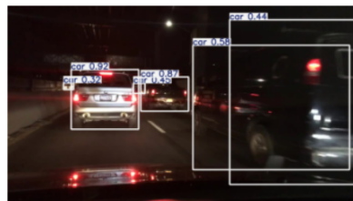
Early Exit 2 IoU: 0.48
