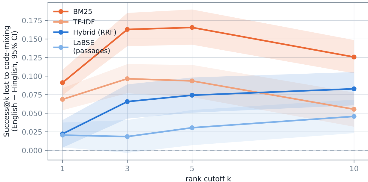
The code-mixing penalty at every depth
