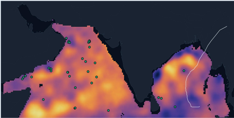
Working prototype: reconstructed temperature at 100 m on 11 May 2023 (held-out year) — dark purple ≈ 17 °C to yellow ≈ 28 °C; green dots = Argo floats; white line = Cyclone Mocha track (IBTrACS)
