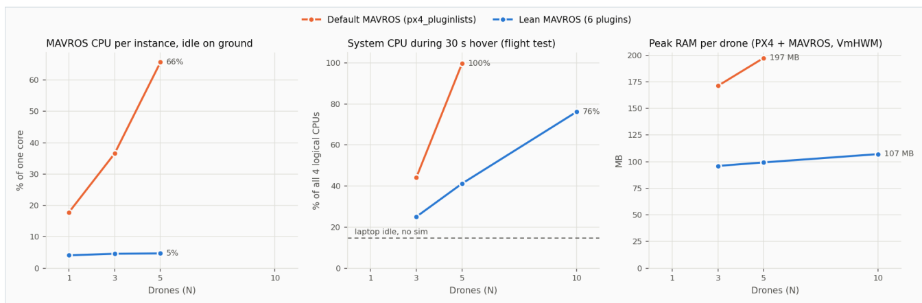
PX4 + MAVROS resources for 3, 5 and 10 drones on this laptop (Phase 1).
