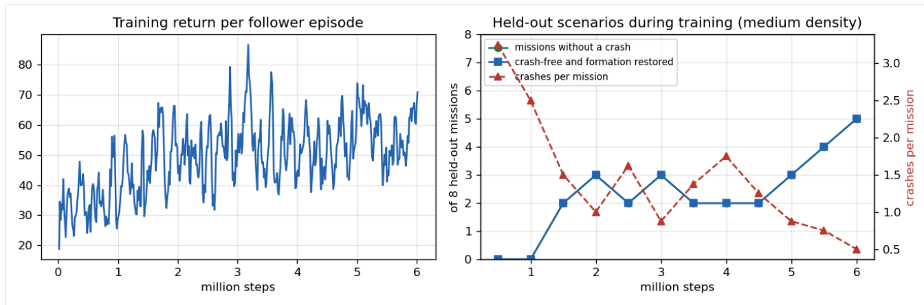
RL training on the laptop: return per episode and held-out scores; still improving at 6 million steps.
