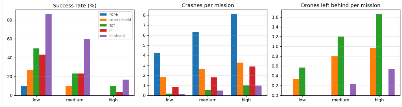
Obstacle avoidance on 90 unseen courses: success rate, crashes and drones left behind for five methods at three obstacle densities.
