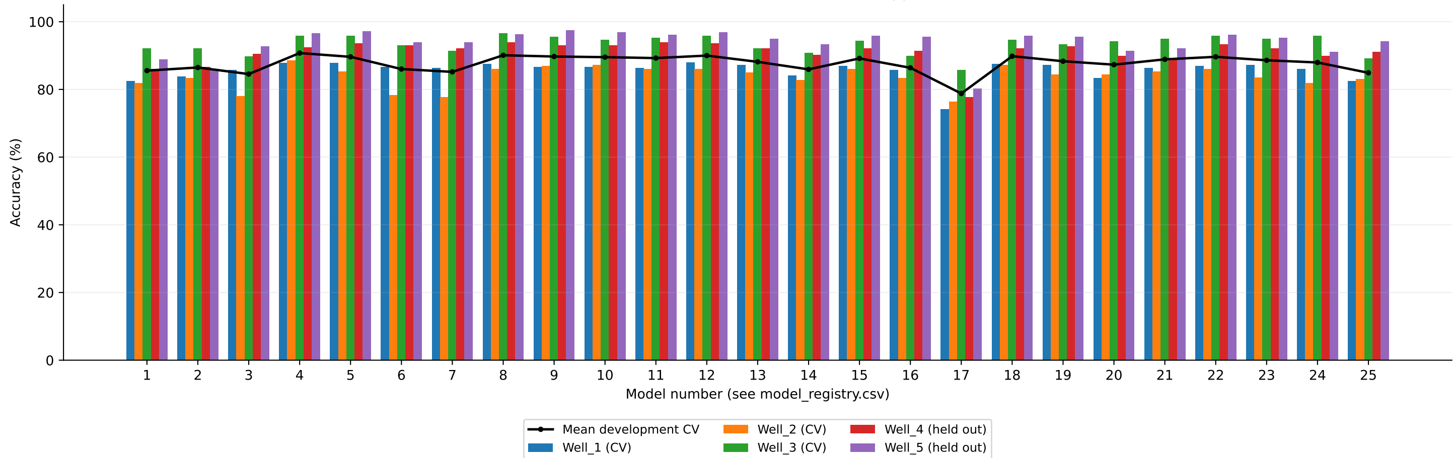
Facies: cross-well validation and held-out application
