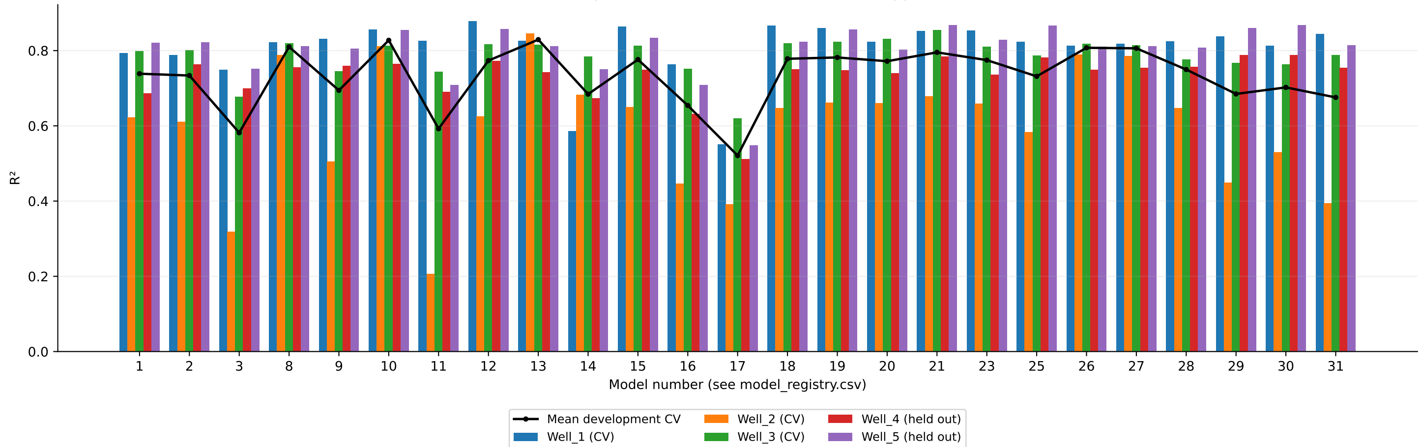
Permeability: cross-well validation and held-out application
