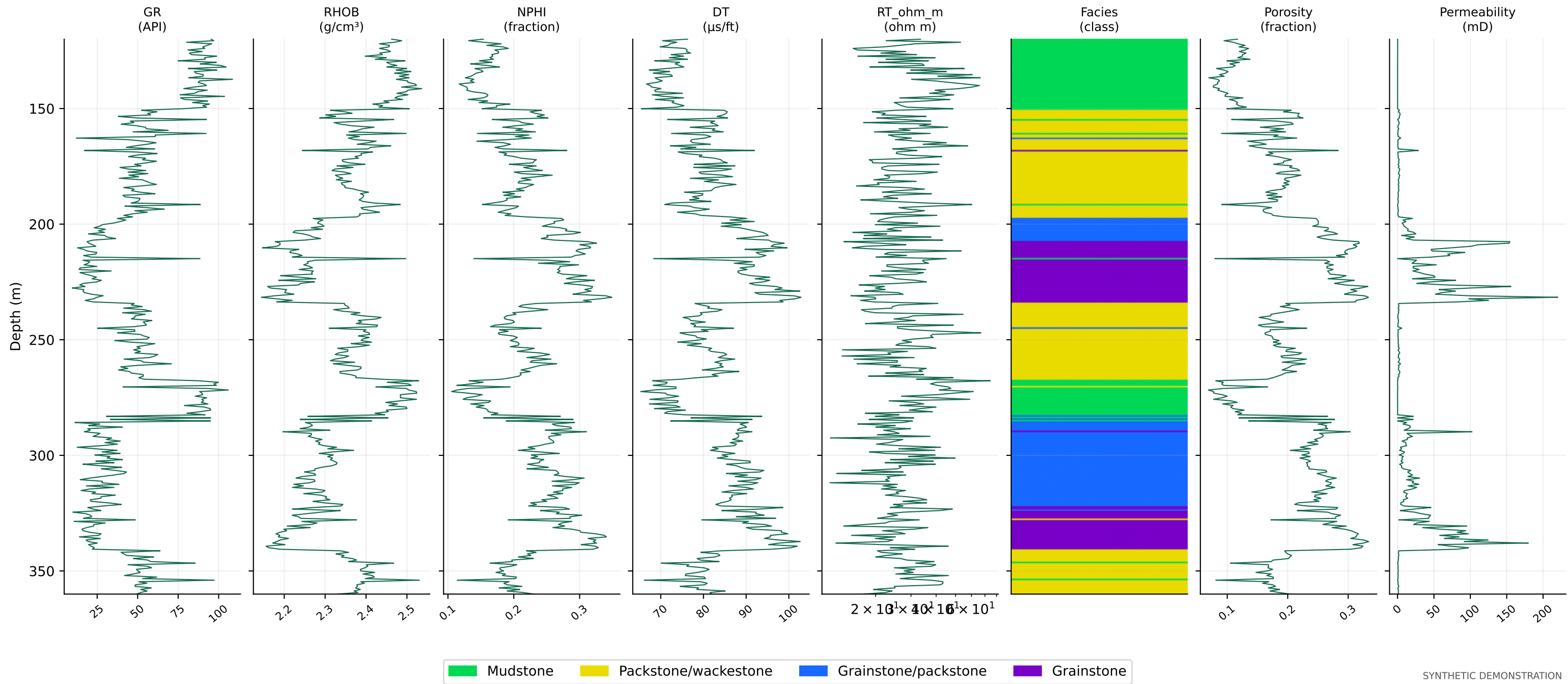
Figure 3. Well logs, facies and laboratory measurements | Well_2
