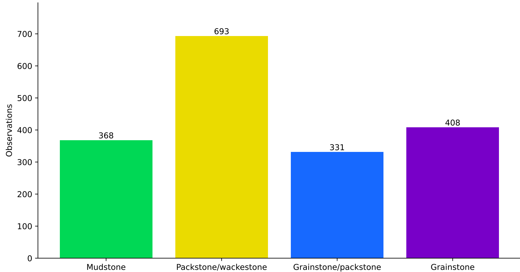
Figure 5. Facies counts
