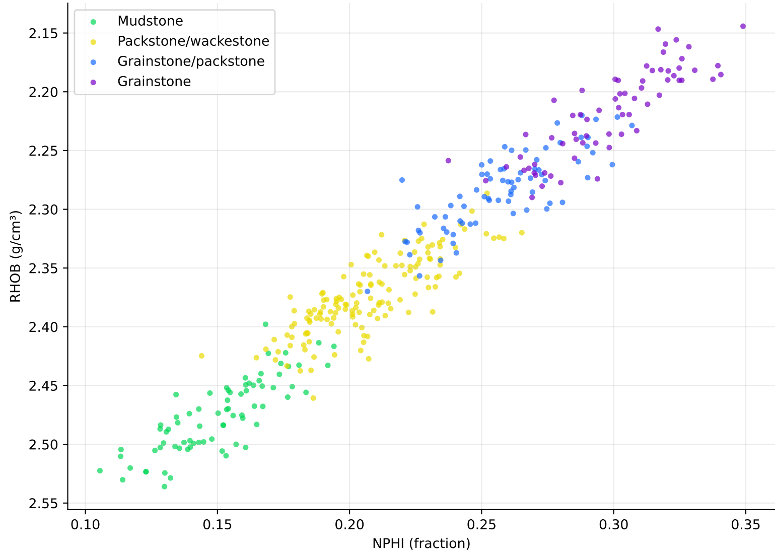
Figure 8. Neutron-density crossplot | Well_2; colored by synthetic facies
