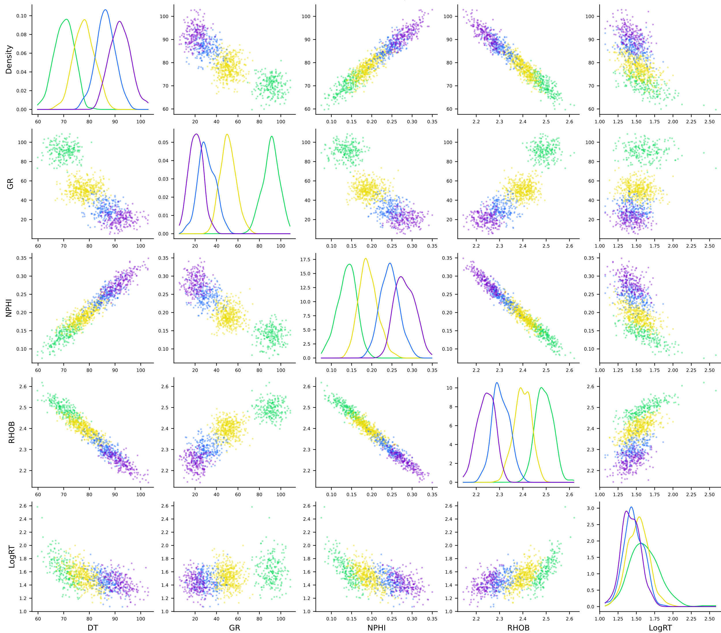
Figure 9. Predictor pairplot by facies | training wells only
