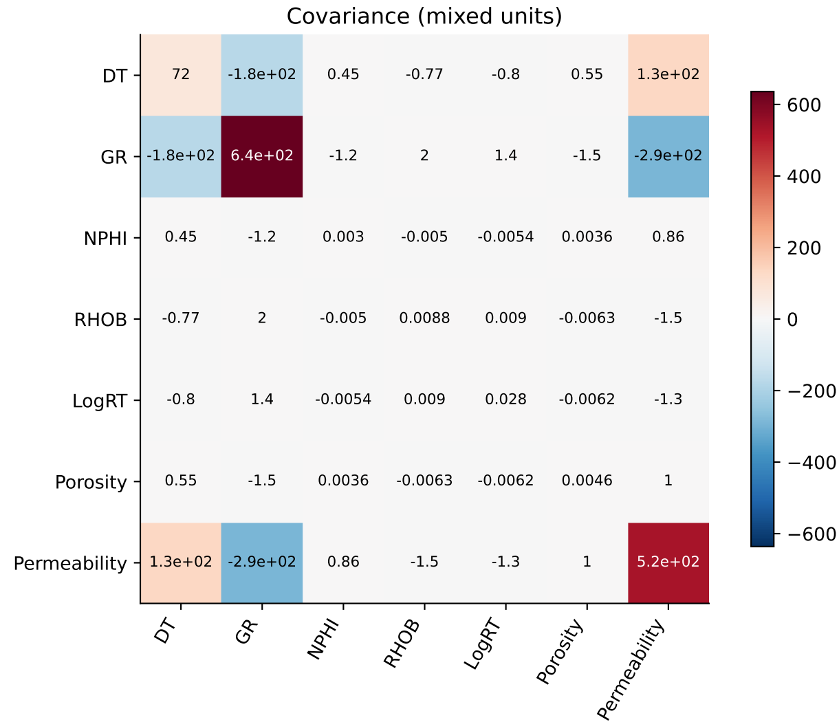
Figure 10. Covariance and Pearson correlation Training wells only; nominal facies codes excluded
