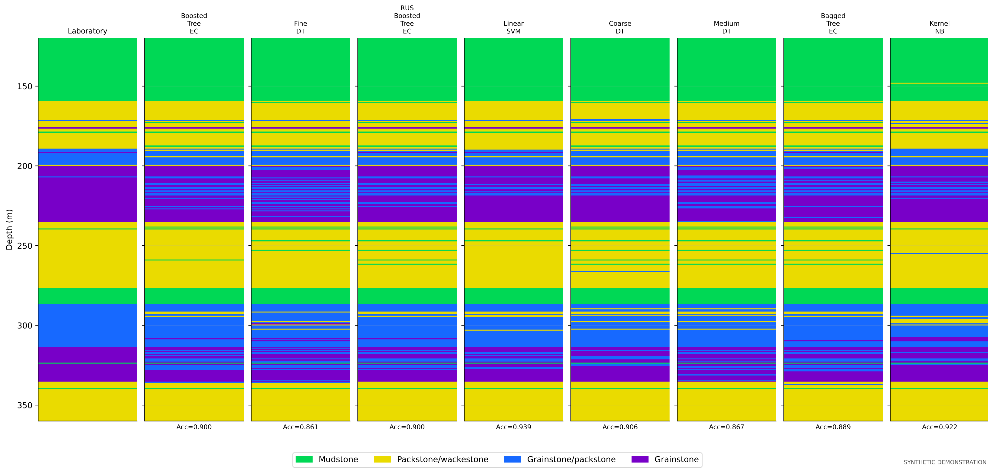
Figure 13. Facies depth tracks | Well_4 held-out test
