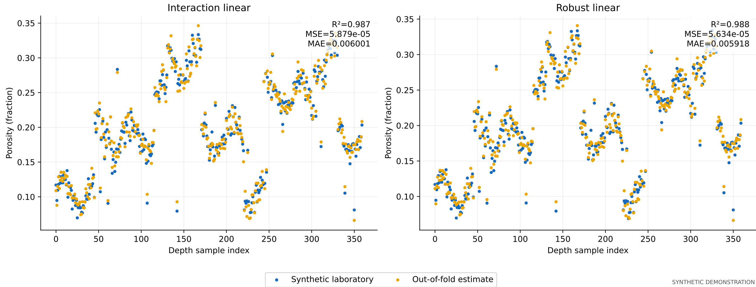
Figure 14. Porosity model point comparisons | Well_2 development validation
