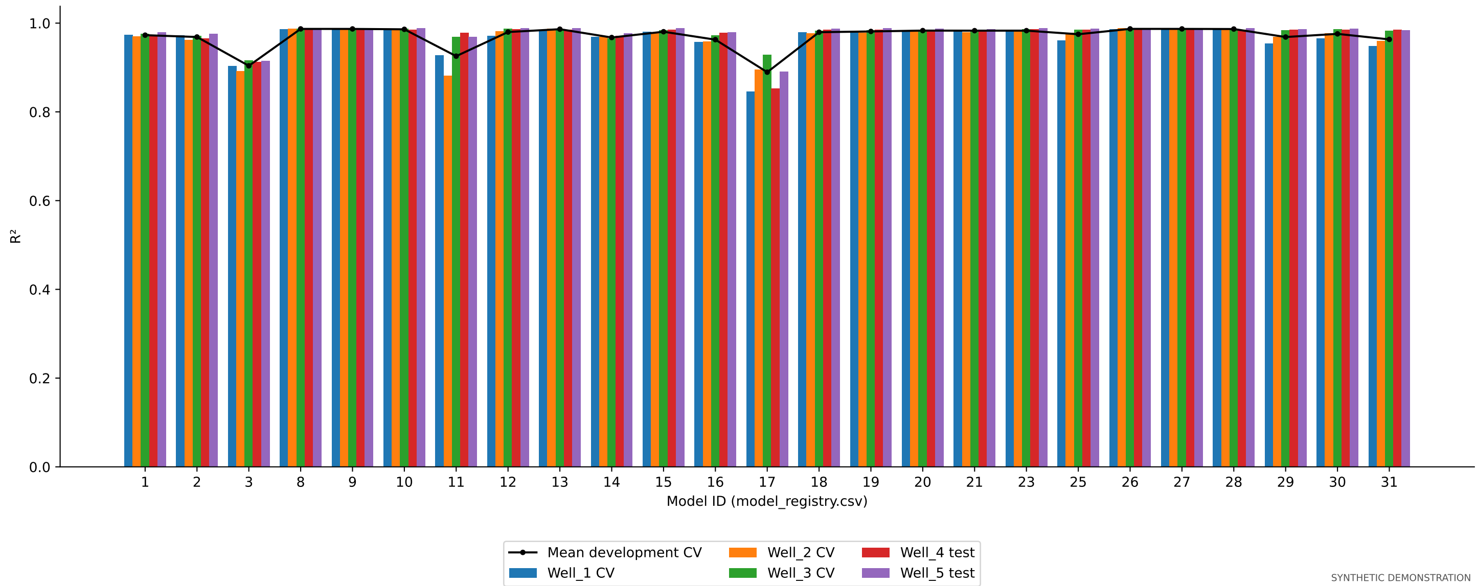
Figure 15. Porosity model comparison
