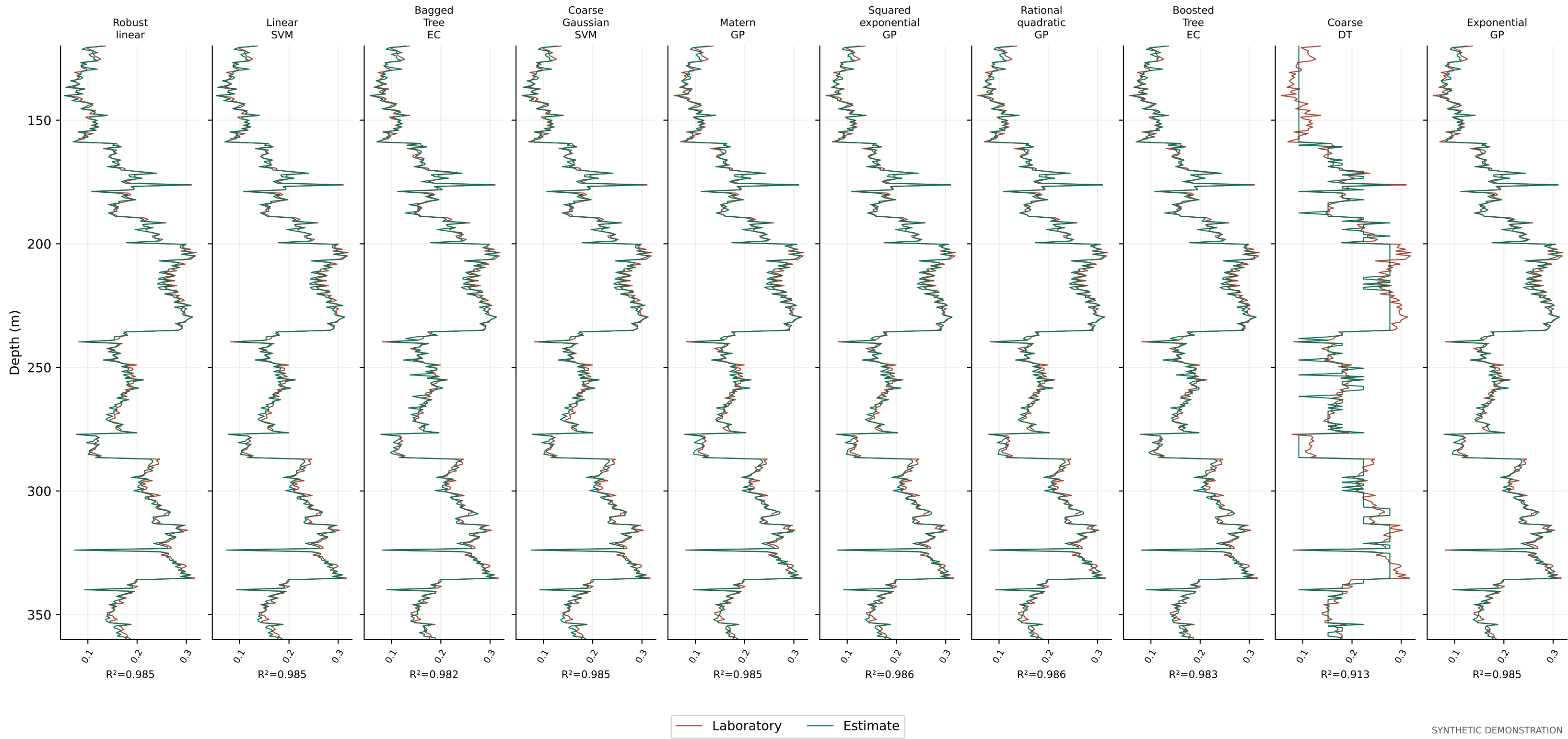
Figure 16. Porosity depth tracks | Well_4 held-out test | fraction
