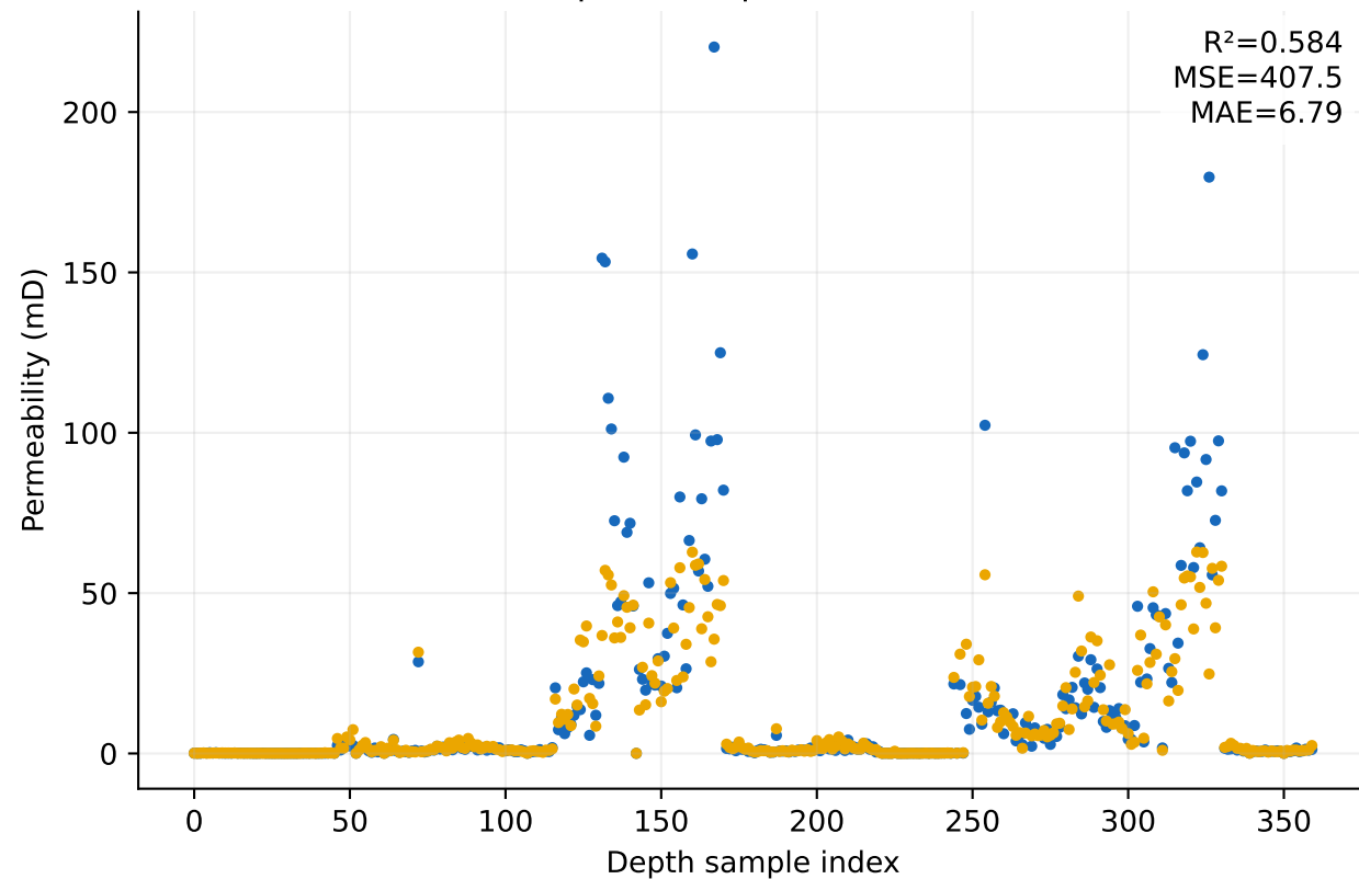
Figure 17. Permeability model point comparisons | Well_2 development validation
