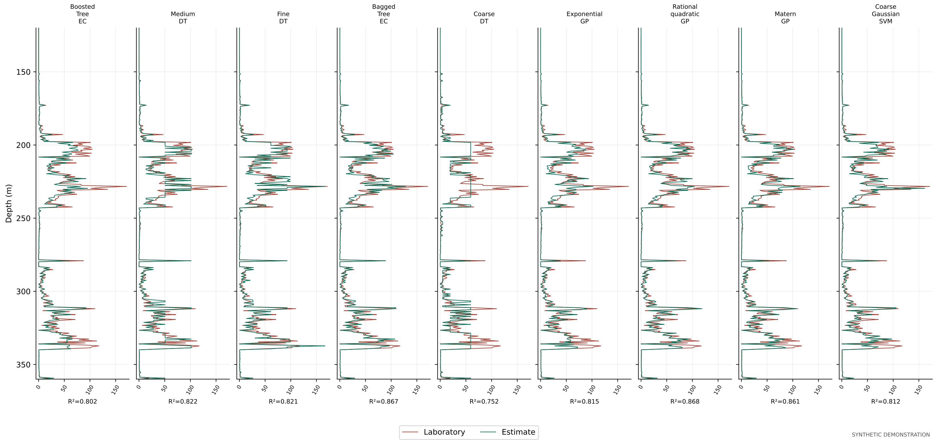
Figure 19. Permeability depth tracks | Well_5 held-out test | mD
