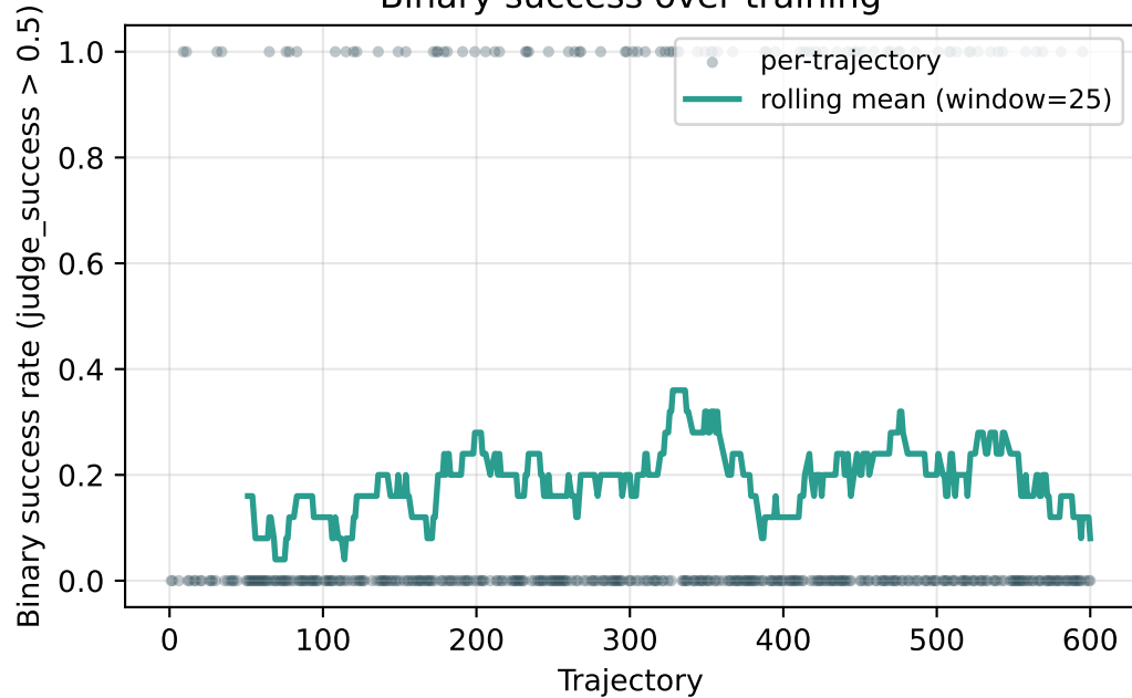
Binary success over training
