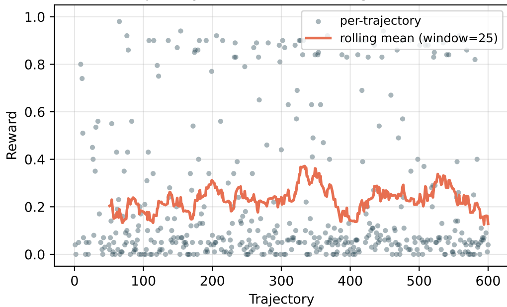
Trajectory reward over training (n=457)
