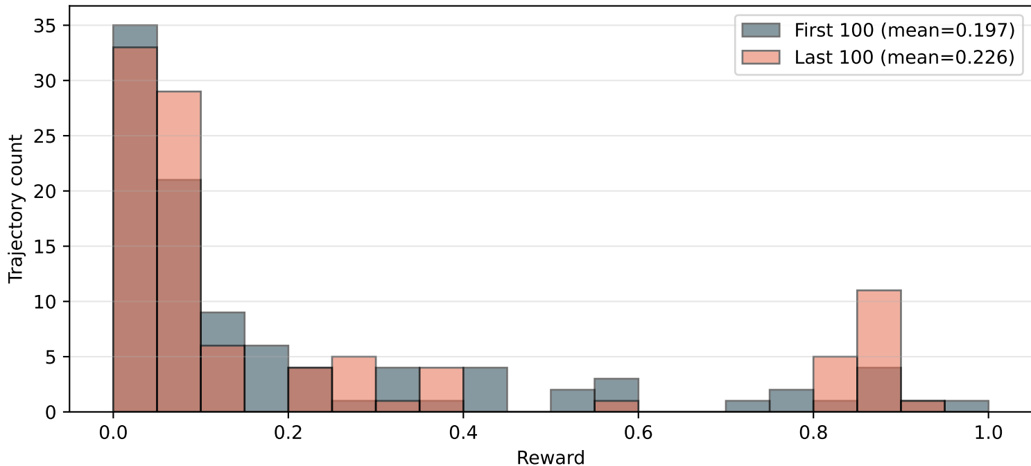
Reward distribution: first 100 vs last 100 trajectories
