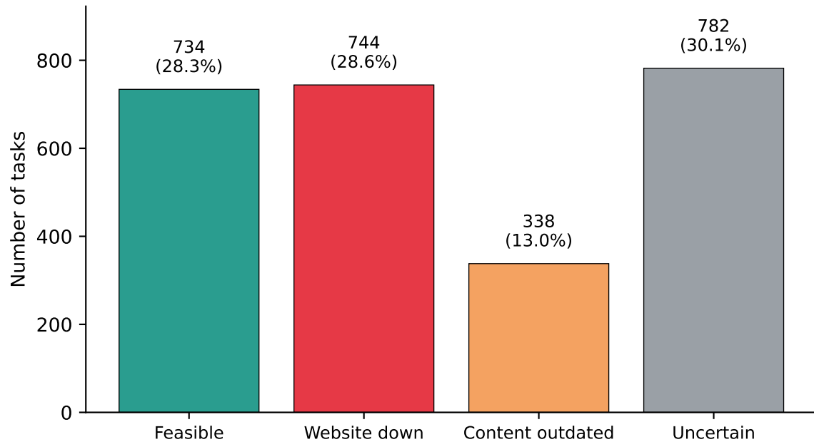
(A) Feasibility classification of 2,598 InSTA tasks
