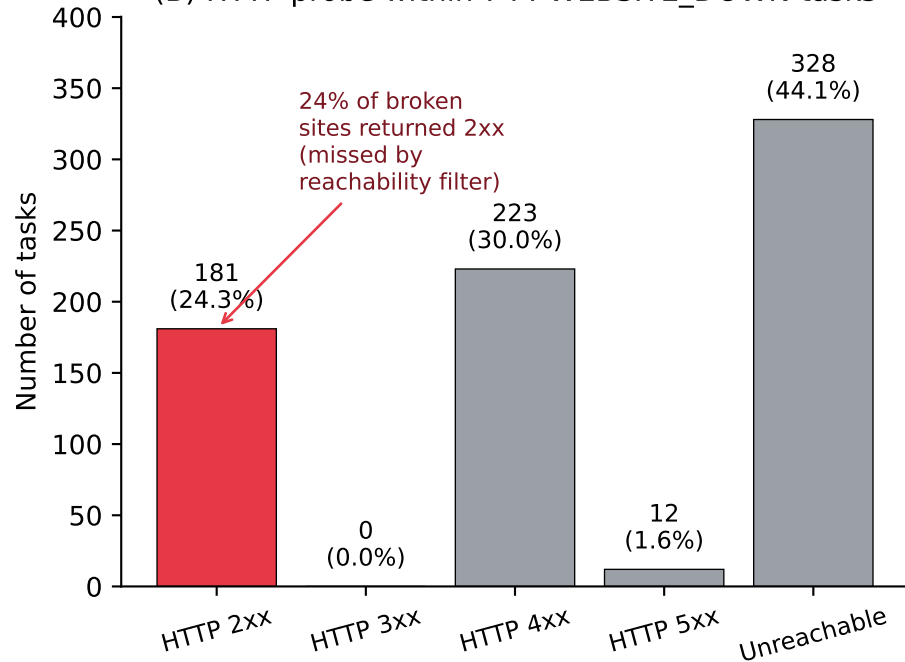
(B) HTTP probe within 744 WEBSITE_DOWN tasks
