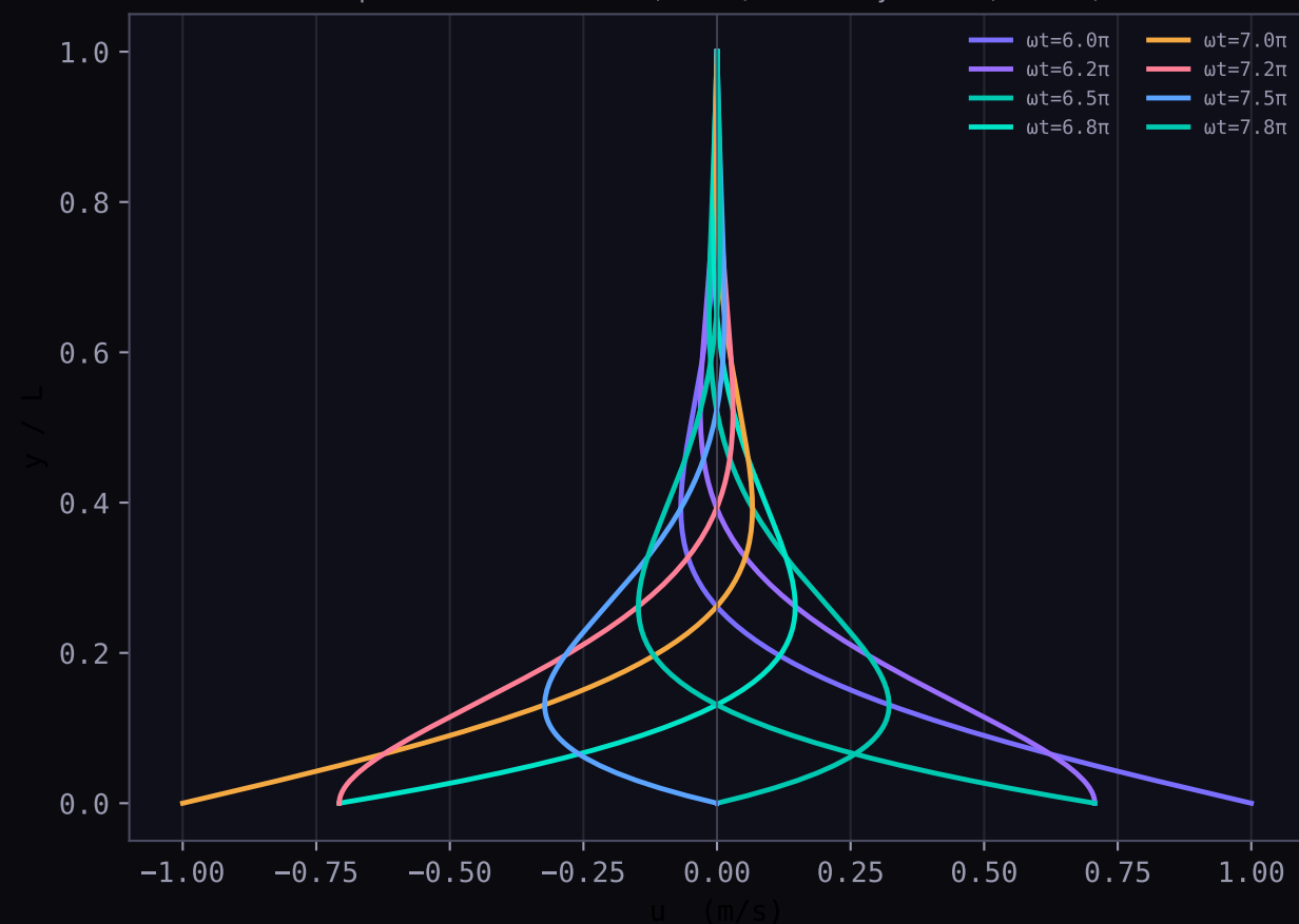
Stokes layer — envelope and penetration depth
