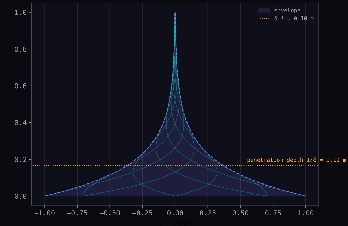
Stokes layer — envelope and penetration depth
