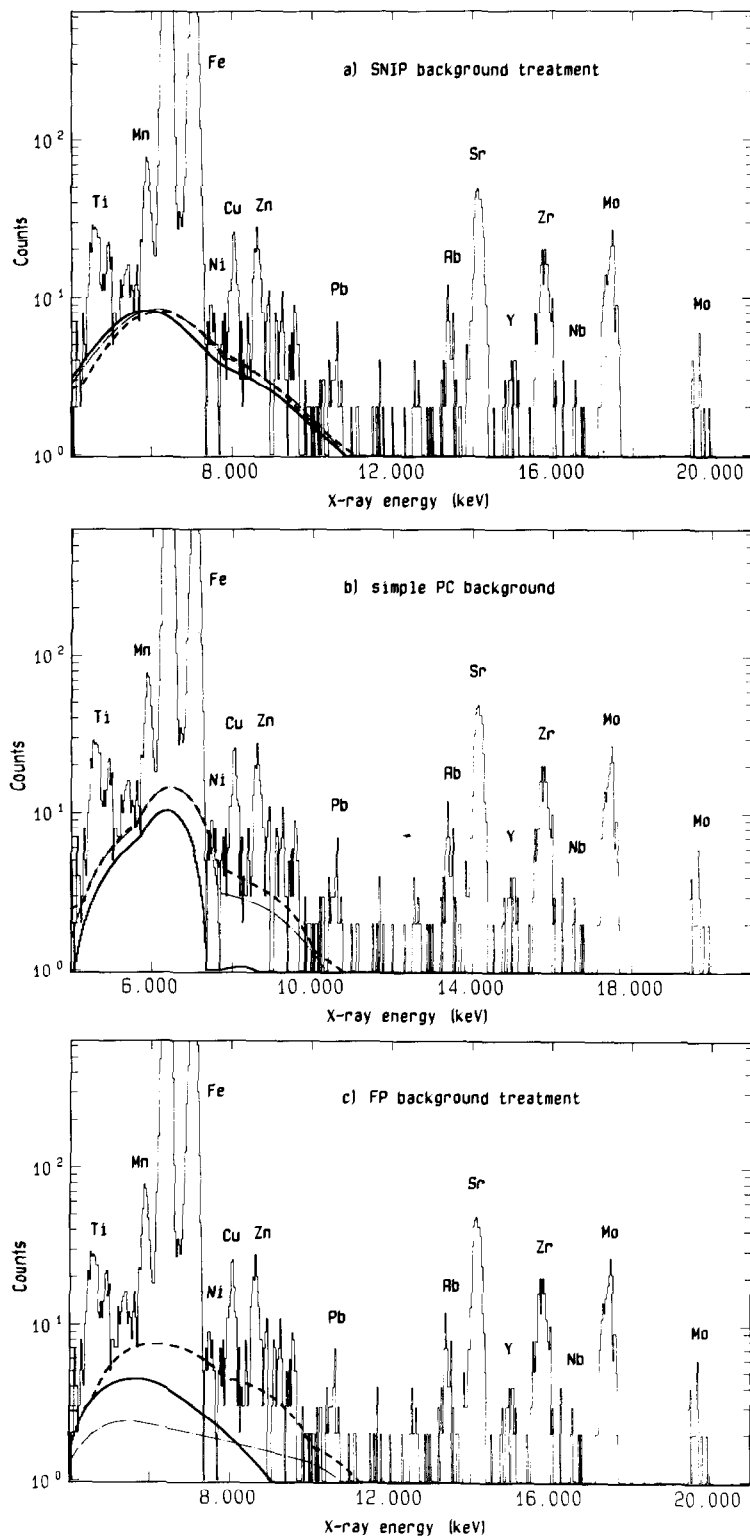
Fig. 3. A typical simulated AGV-1 spectrum representing Q = 0.14 \mu\text{C} showing as thick solid curves the a) SNIP background, b) PC background, and c) FP background approximations. Also shown are the backgrounds calculated for a Q = 1.4 \mu\text{C} spectrum (dot-dash curves, scaled by 0.1) and the Q = 14 \mu\text{C} spectrum (dashed curves, scaled by 0.01).
