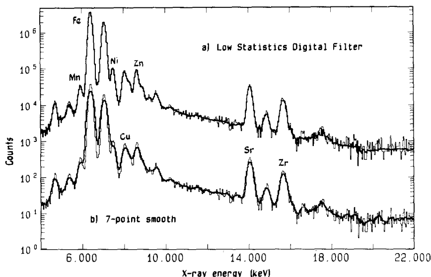
Fig. 1. PIXE spectrum from a mineral grain (augite), processed with a) the Low Statistics Digital Filter (offset \times 100 for clarity), and b) a spectrum smoothing algorithm using 7-point means.
