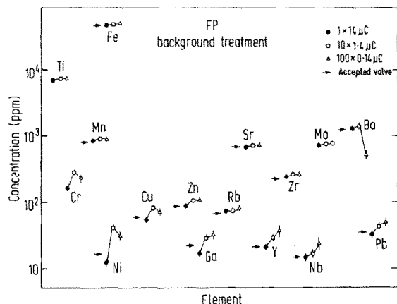
Fig. 6. Concentrations deduced from the parent AGV-1 spectrum using the FP background treatment, and the averages of concentrations deduced from the simulated spectra (symbols as in fig. 4).
