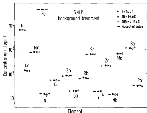
Fig. 4. Concentrations deduced from the parent AGV-1 spectrum using the SNIP background treatment (solid symbols), and the averages of concentrations deduced from the simulated spectra (open squares, average of 10 spectra of Q = 1.4 \mu\text{C} each, and open triangles, average of 100 spectra of Q = 0.14 \mu\text{C} each).
