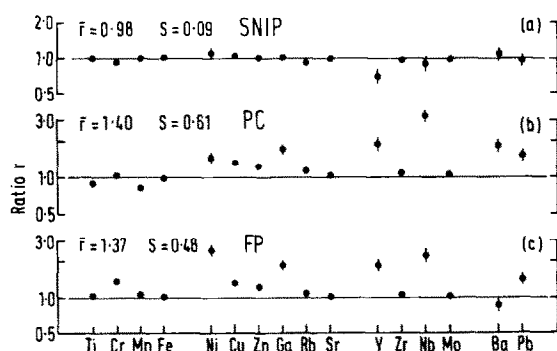
Fig. 7. The ratio r , for each element, of the average concentration deduced from the 100 spectra of Q = 0.14 \mu\text{C} each to the concentration deduced from the parent spectrum, using the a) SNIP, b) PC and c) FP background treatments.
