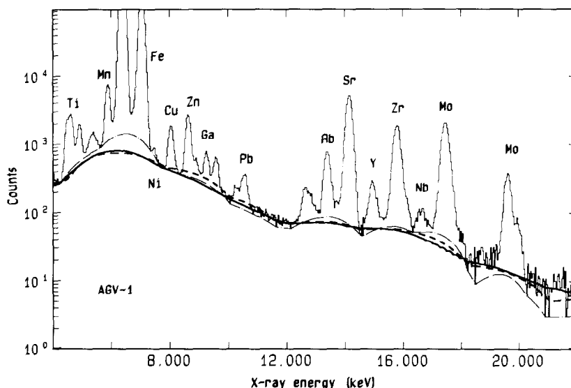
Fig. 2. PIXE spectrum from the AGV-1 glass (3 MeV protons, Q = 14 \mu\text{C} ) showing the SNIP background (thick solid curve), the PC background (dot-dash curve), and the FP background (dashed curve).
