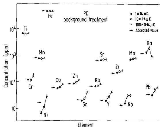
Fig. 5. Concentrations deduced from the parent AGV-1 spectrum using the PC background treatment, and the averages of concentrations deduced from the simulated spectra (symbols as in fig. 4).
