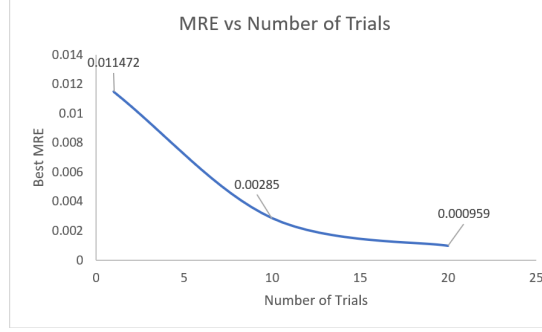
Figure 6.5: MRE and Number of Trials
