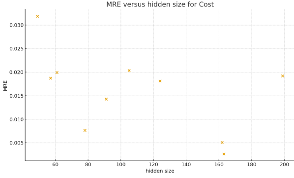
(a) MRE vs Hidden Layer Size: Cost
