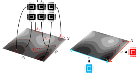
Figure 2.1: Level Set Partitioning (left) and Variable Partitioning (right) [8]
