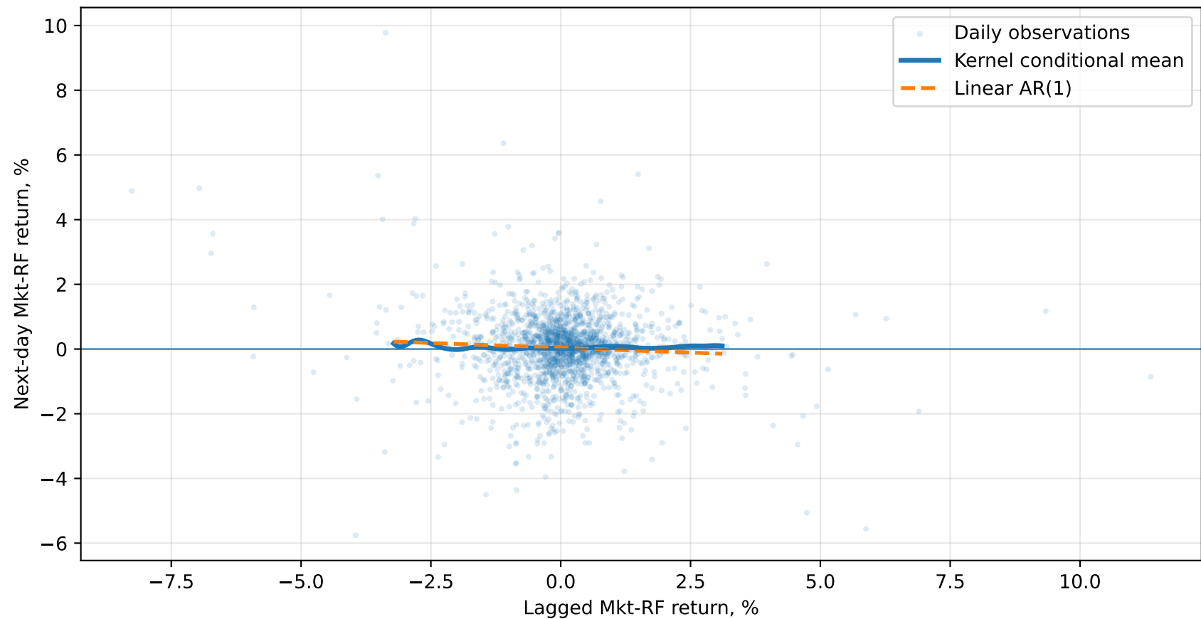
Conditional mean: almost linear at the center, unstable in the tails
