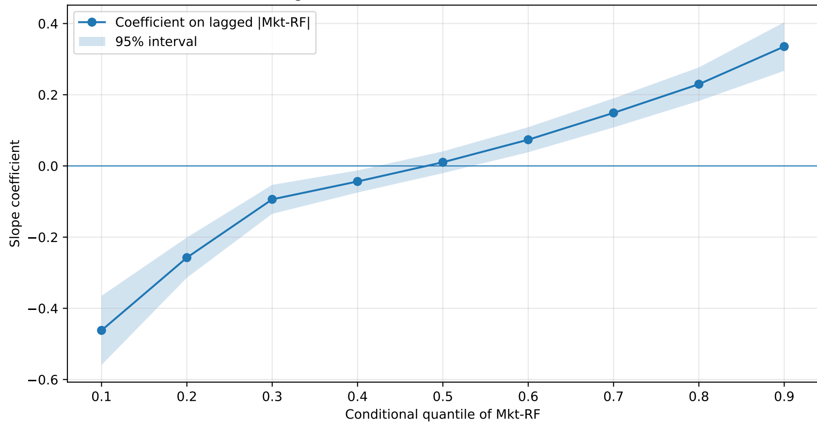
Quantile regression: nonlinear effects across the distribution
