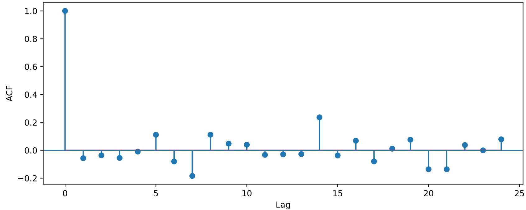
ACF of OLS residuals - inertial Taylor rule
