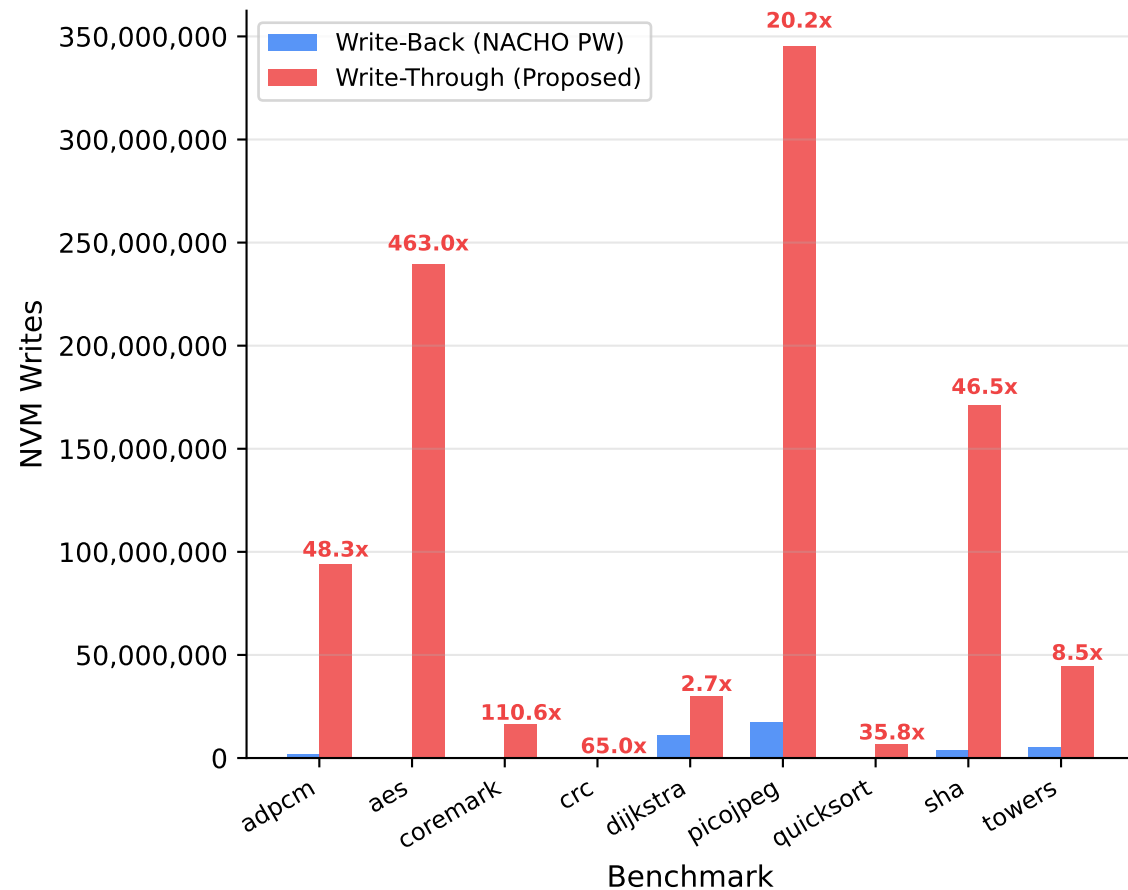
NVM Write Count (lower is better)
