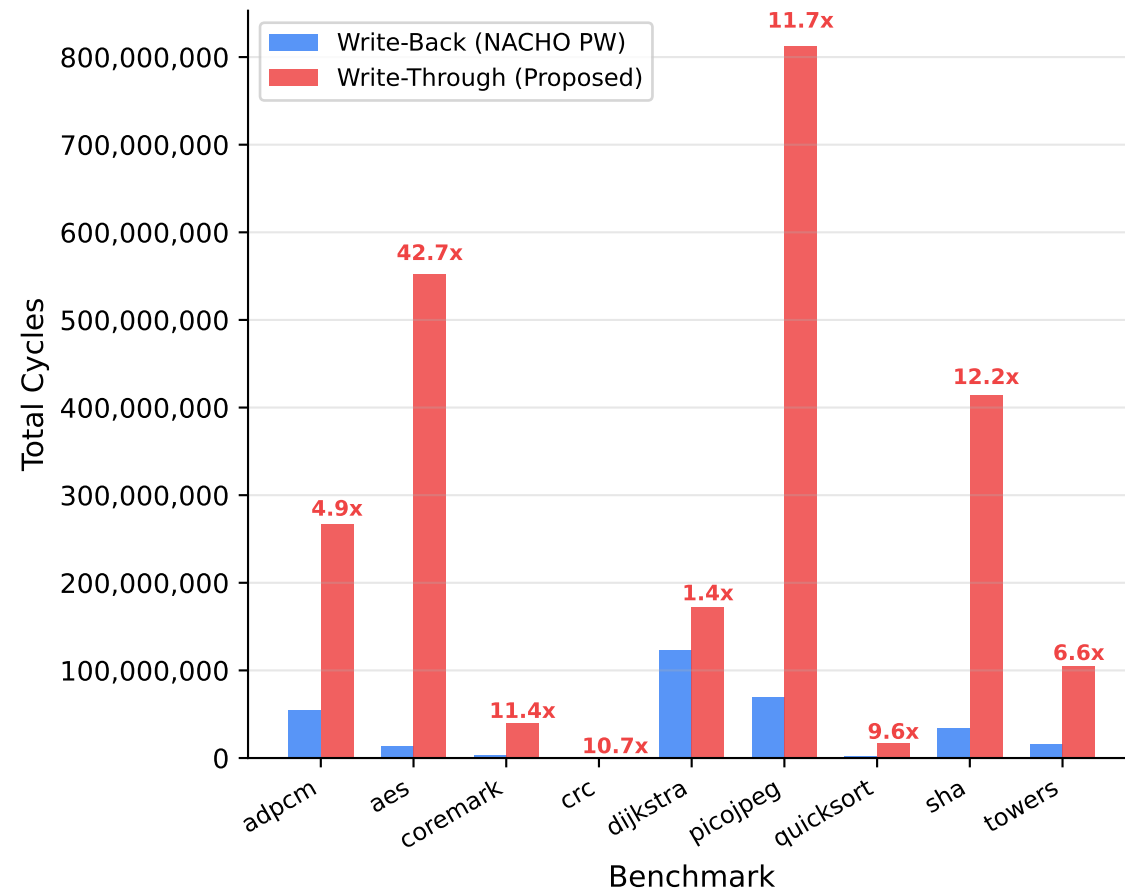
Execution Cycles (lower is better)
