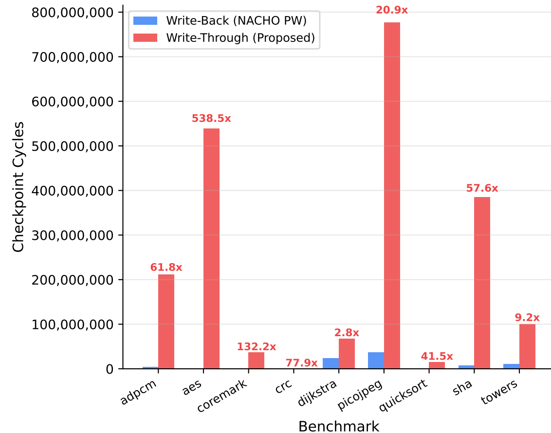
Checkpoint Overhead Cycles (lower is better)
