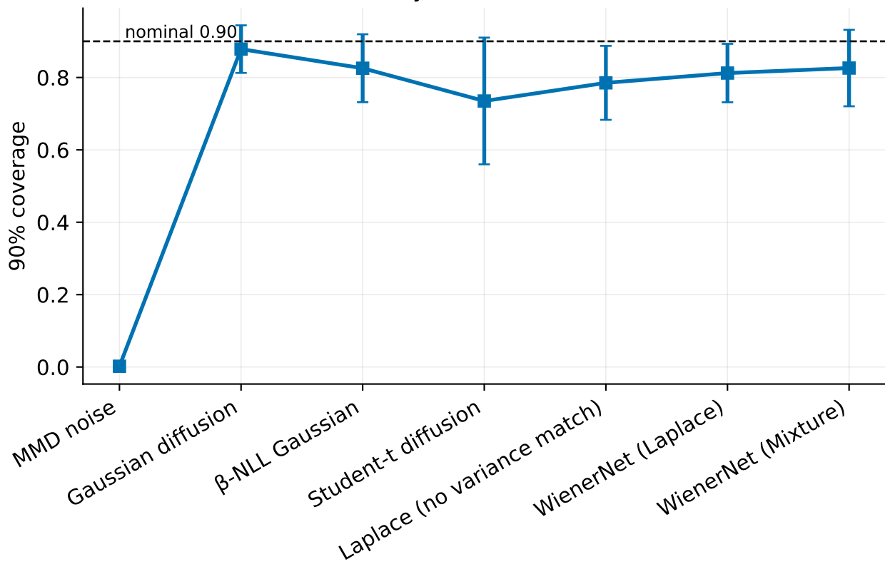
Noise-family ablation — calibration
