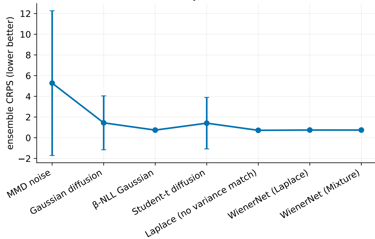
Noise-family ablation — skill
