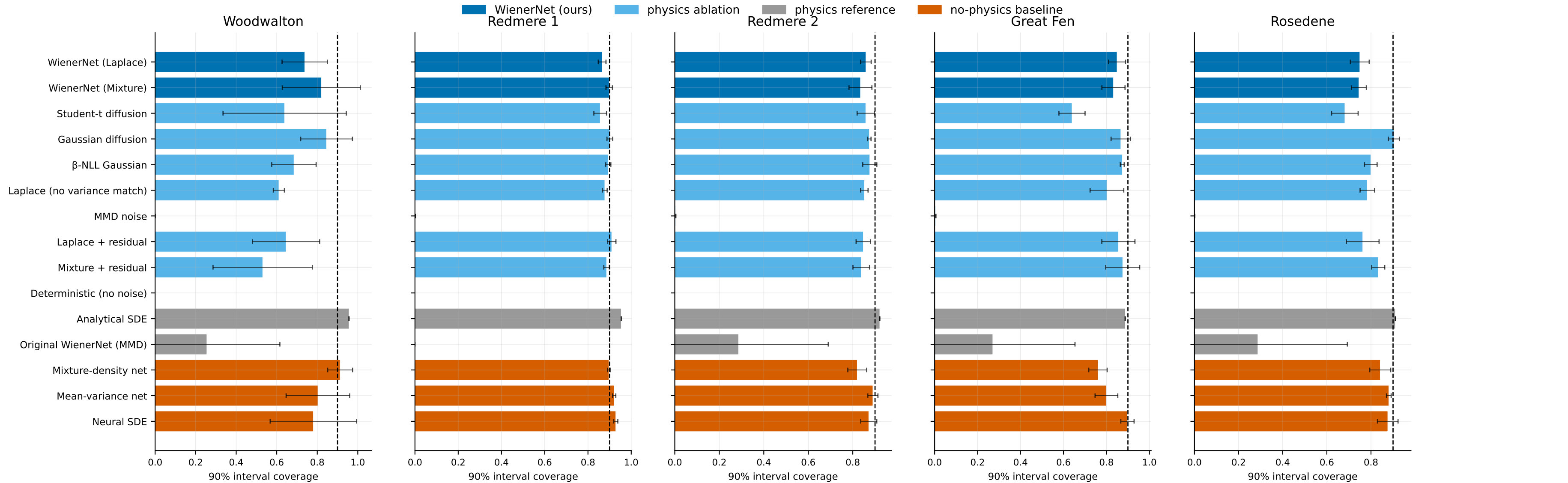
All models — 90% coverage per held-out site (dashed = nominal)
