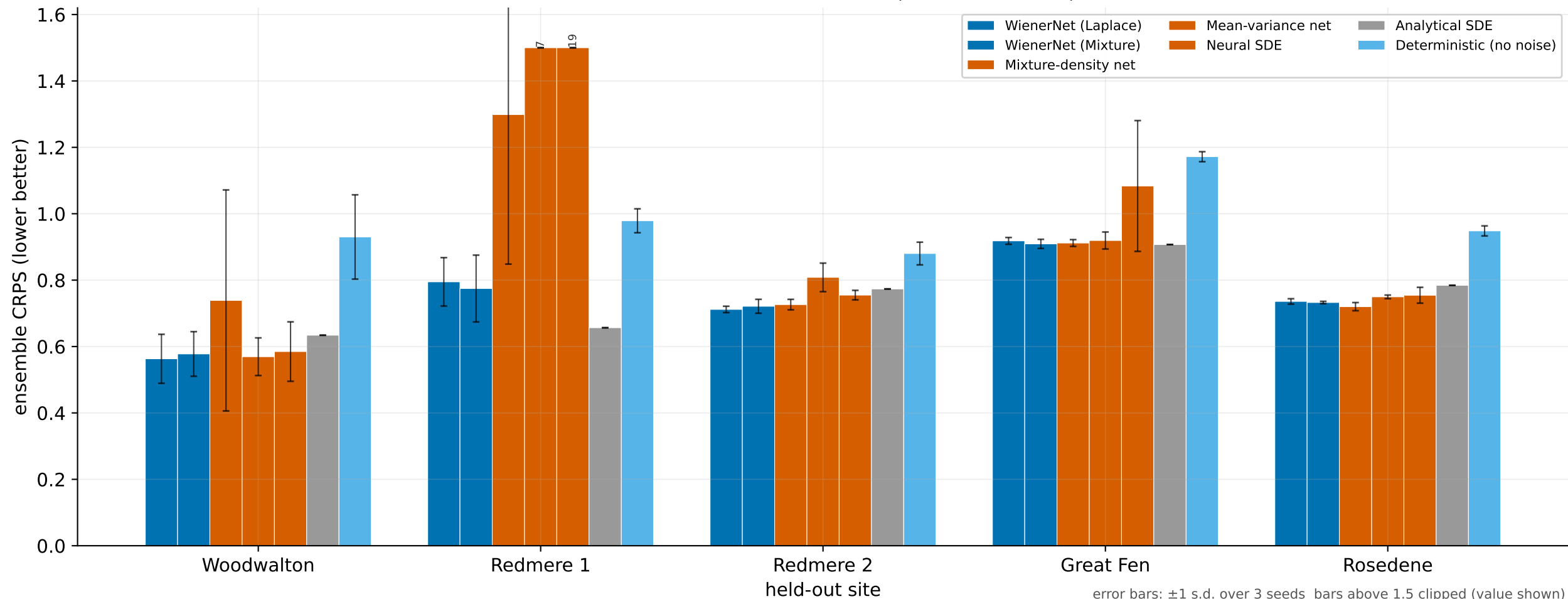
Predictive skill on held-out sites (headline models)
